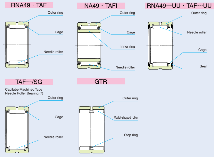
Structures of Machined Type Needle Roller Bearings
